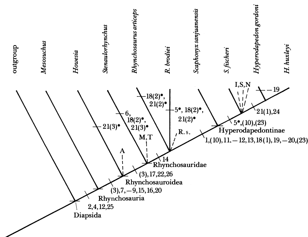
FIGURE 43. The most parsimonious cladogram showing the relationships of the nine best-known taxa of rhynchosaurs, based on a cladistic analysis by the PAUP program of 26 characters (see text and table 7). The length of the tree is 35 steps; CI is 0.857. Postulated parallelisms are indicated by an asterisk, postulated reversals by a negative sign, uncertainly placed characters by parentheses, and derived character states by (1), (2) or (3). Seven less-well-known taxa have been added to the core cladogram (see text). Abbreviations: A, Acrodonta ; I, Isalorhynchus ; M, Mesodapedon ; N, Nova Scotia rhynchosaur; R.s., Rhynchosaurus spenceri ; S, Supradapedon ; T, Texas rhynchosaur.
